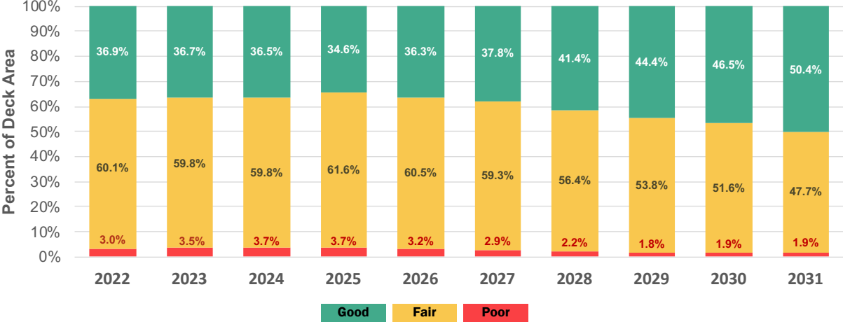
Figure 4-2. NHS Bridge Performance Projection – Desired Scenario
